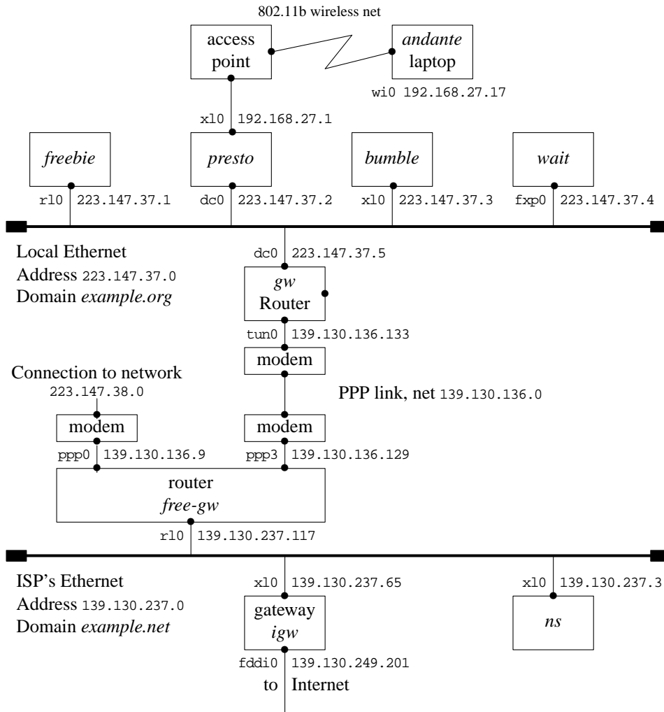
Figure 16-7: Reference network
