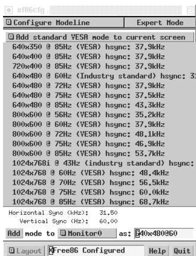
Figure 6-17: xf86cfg VESA mode lines
