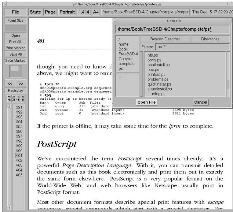
Figure 15-2: gv display
