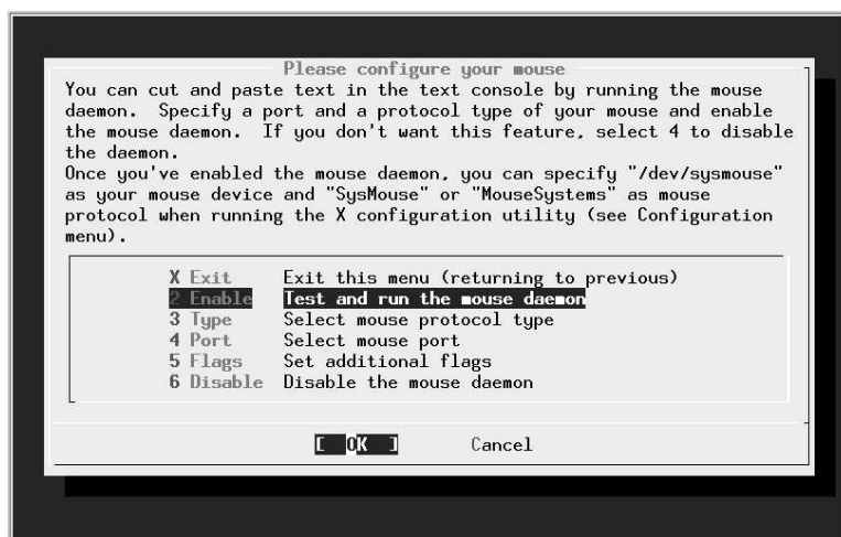
Figure 6-8: Mouse menu
