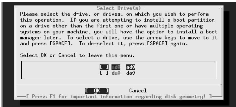
Figure 5-4: Disk selection menu
